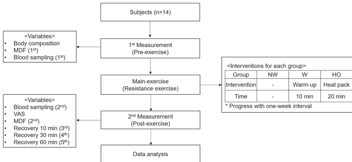
Fig. 1. Flow chart.
